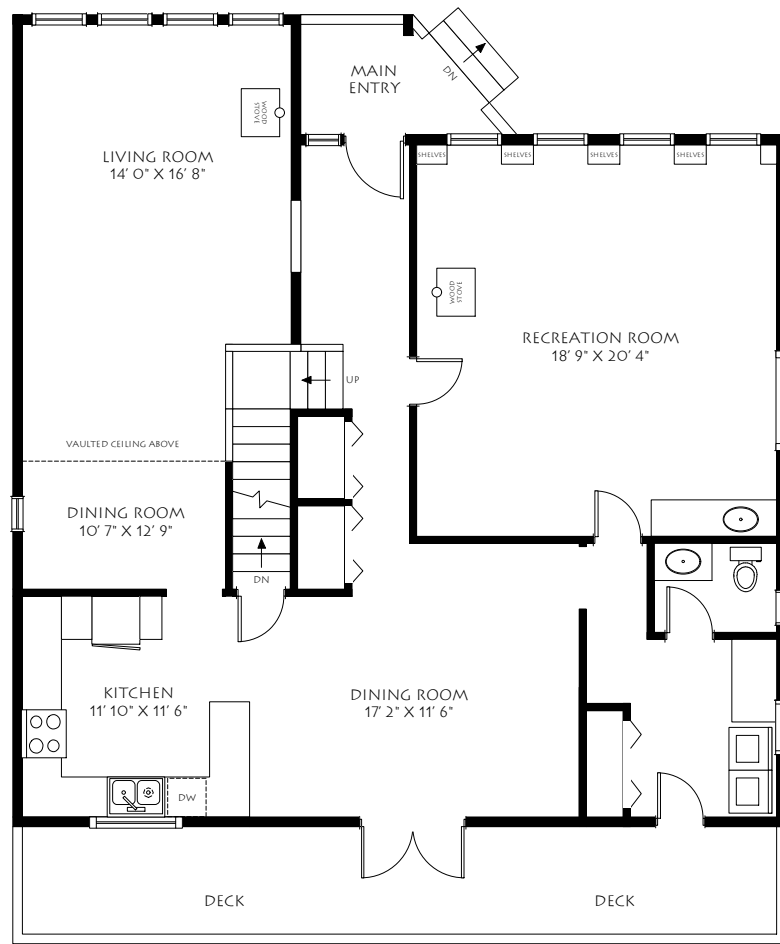
MAIN FLOOR
