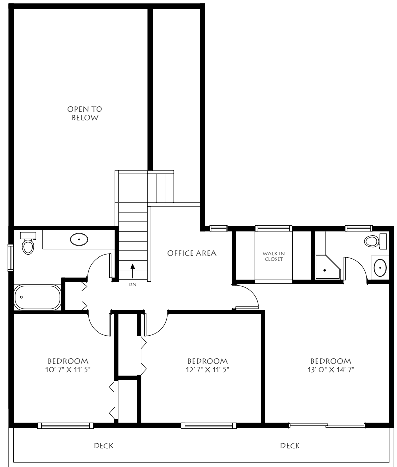
SECOND FLOOR
